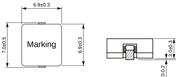
Dimensions: [mm]
