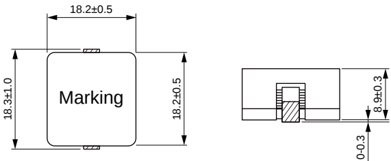
Dimensions: [mm]
