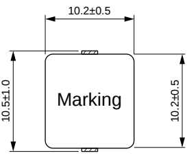
Dimensions: [mm]
