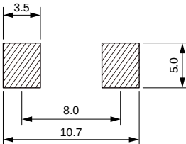
Land Pattern: [mm]
